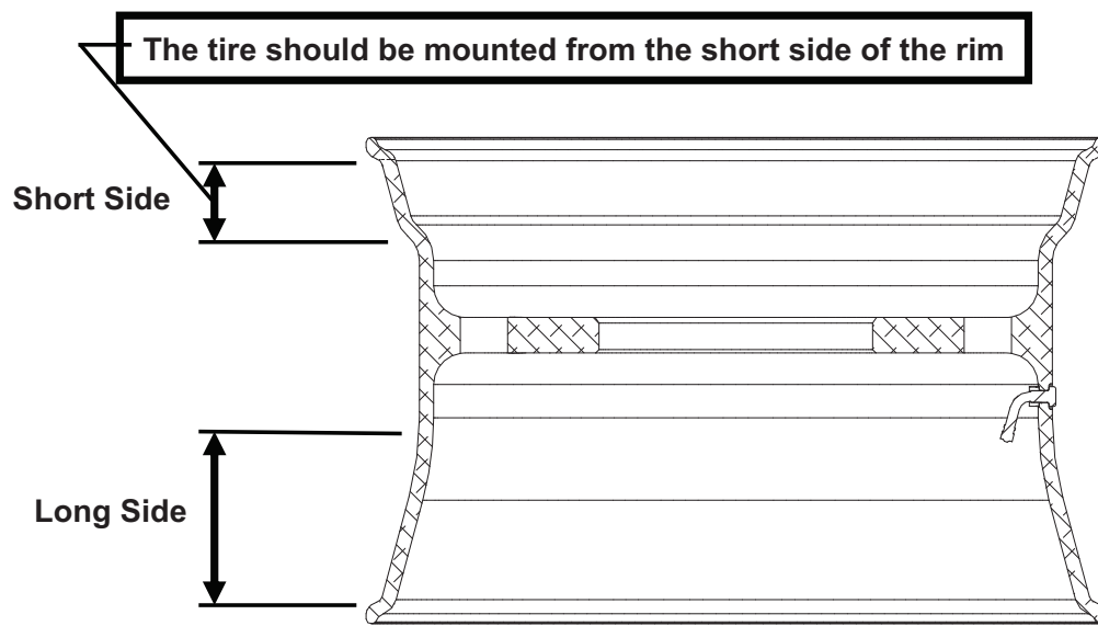
29660 Aluminum Wheel
