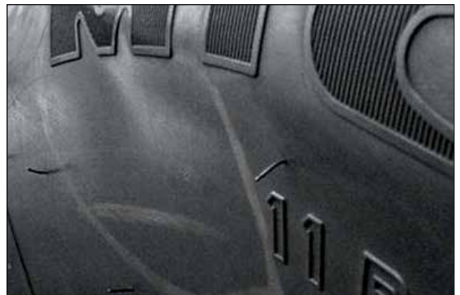
Ripples or Bulges in the Sidewall Flex Area
