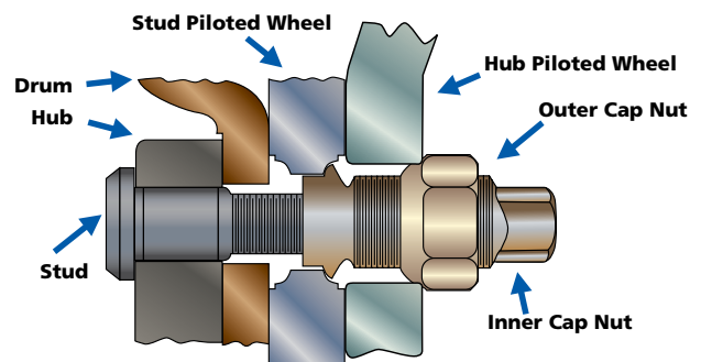
Figure 1: Improper Mounting
