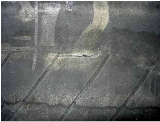
EFFECT: Inner Liner Cut CAUSE: Shipping or Mounting Damage
