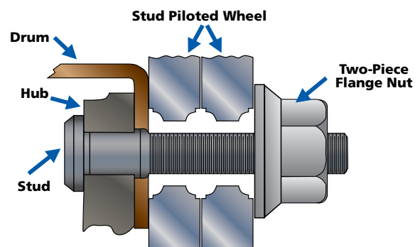
Figure 2: Improper Mounting
