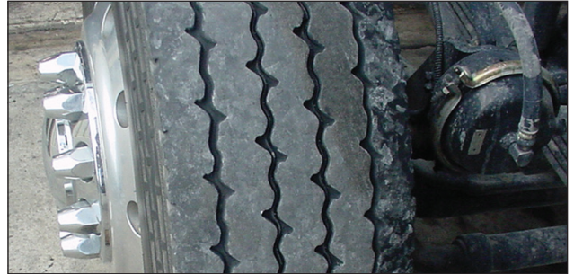
Camber Wear
