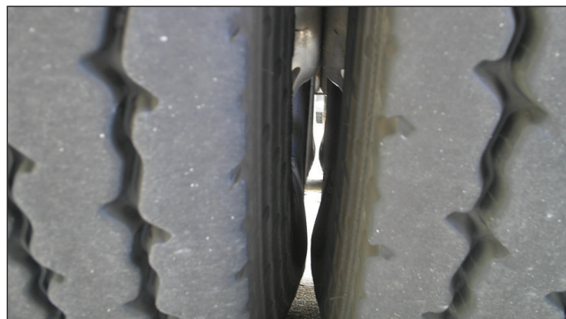
EFFECT: Friction Severely Weakens the Casing CAUSE: Dual Kissing
